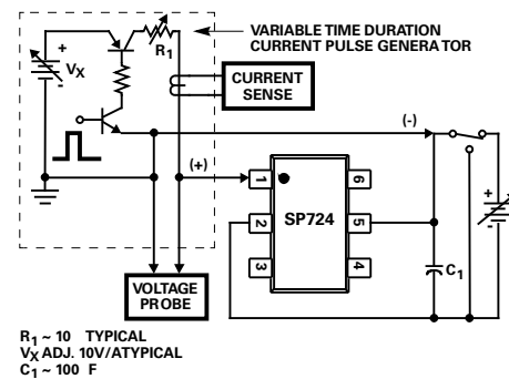
TYPICAL SP724 PEAK CURRENT TEST CIRCUIT WITH A VARIABLE PULSE WIDTH INPUT
